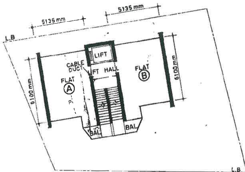
5th TO 21th FLOOR PLAN
